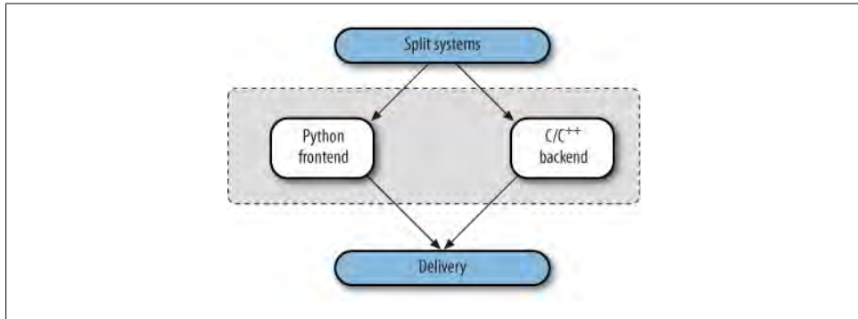
Figure 21-4. Hybrid designs
