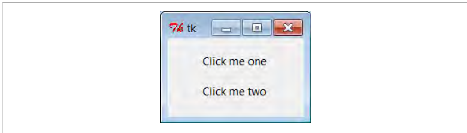
Figure 9-28. Canvas-bind window
